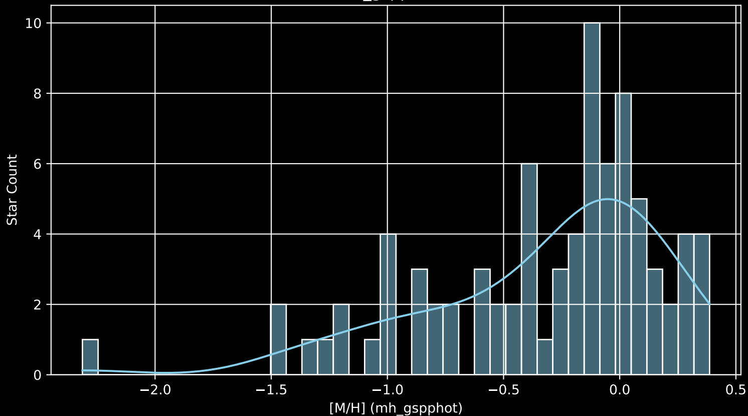
APOGEE DR17 Field: [002+04] [M/H] (mh_gspphot) (n= 82)
