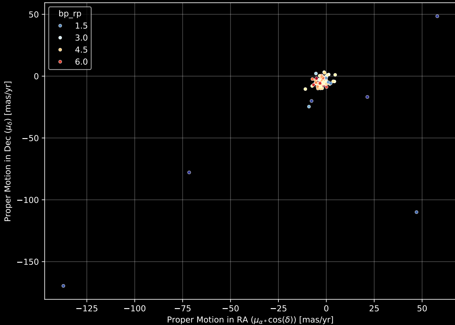
APOGEE DR17 Field: [002+04] Proper Motion Diagram (n= 86)
