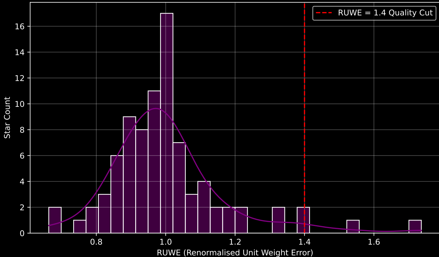
GAPOGEE DR17 Field [002+04] RUWE Distribution (n= 85)
