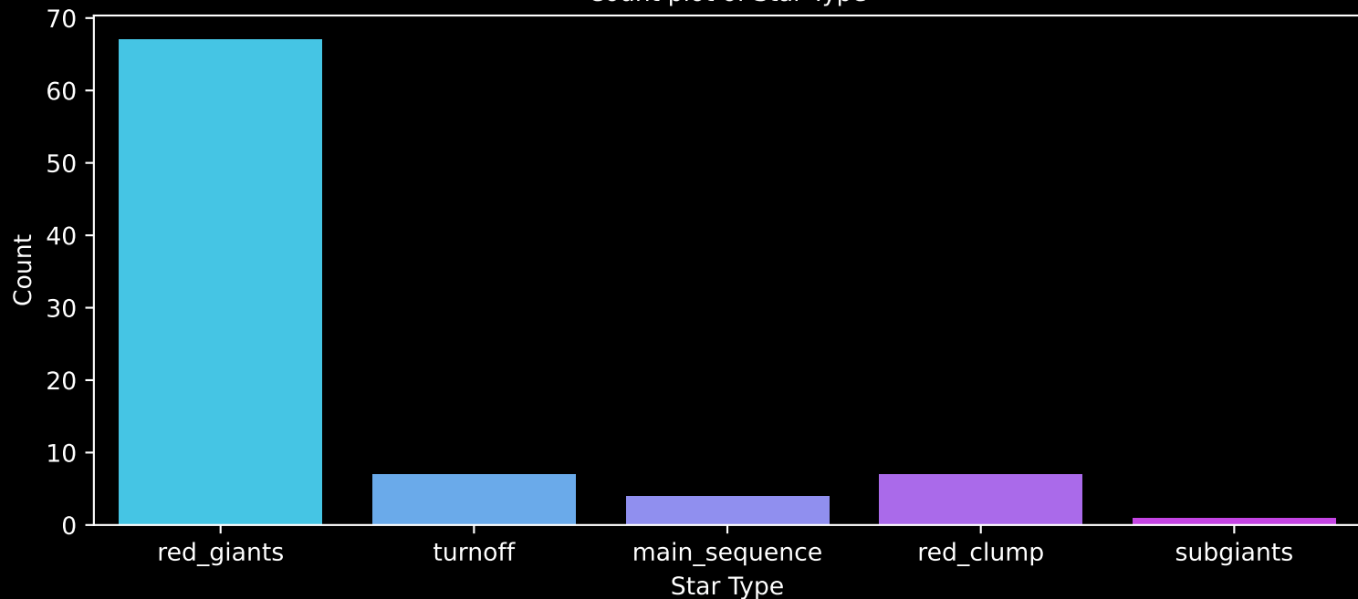
APOGEE DR17 Field: [002+04] Count plot of Star Type
