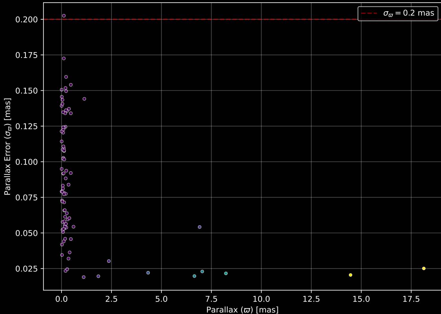
APOGEE DR17 Field: [002+04] Parallax Quality (n= 86)
